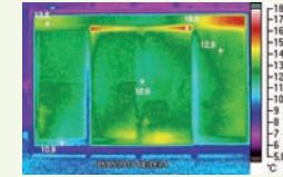
Standard aluminium frame and 44/2 glazing*
